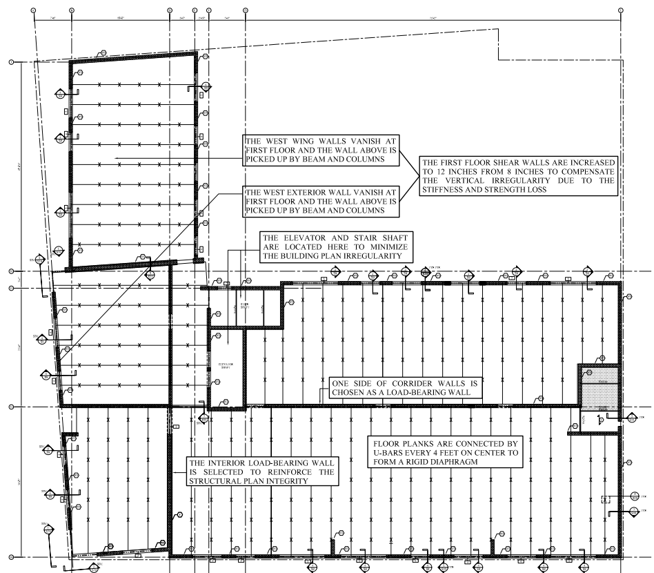
Figure 5: Typical floor plan.
