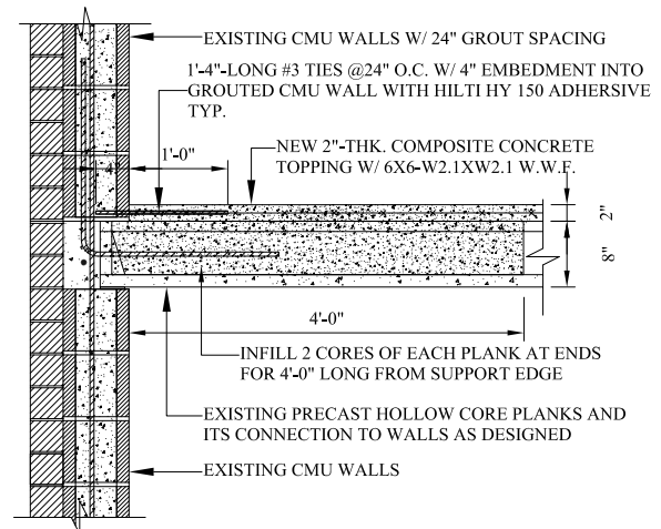
Figure 4: Plank strengthening.
