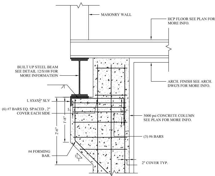
Figure 3: Corbels for wall set-back.
